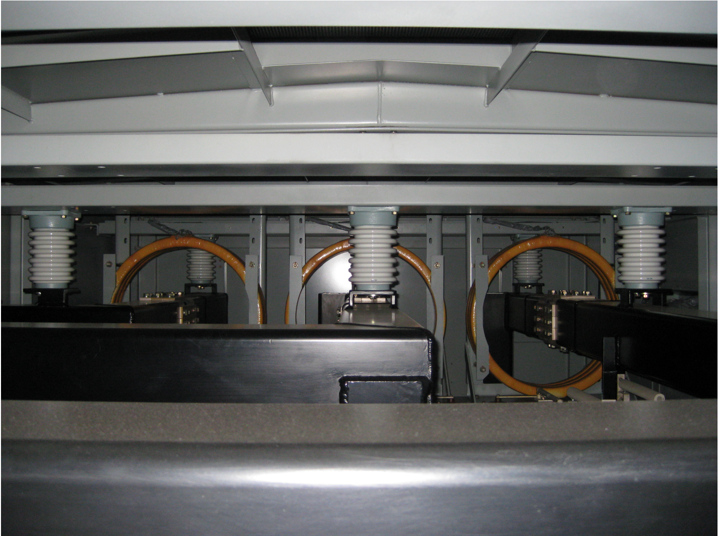
Terminal Ends of Windings with Terminal CTs
